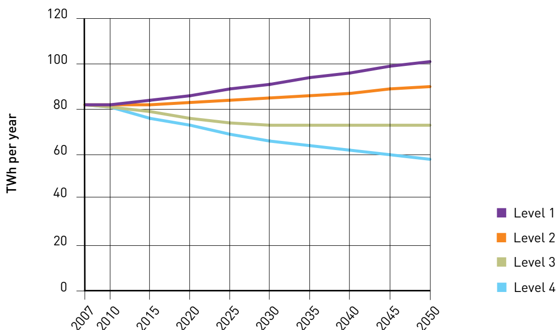
Figure A4: Trajectories for non-domestic lighting and appliances under four levels of change
