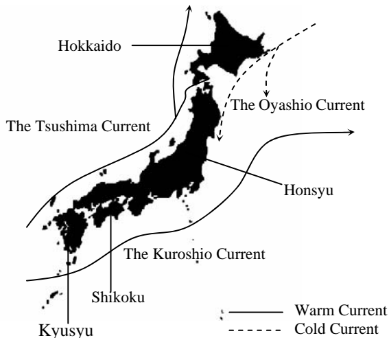
Fig. 5 Ocean Currents around Japan
