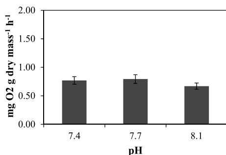
Fig. 3. Effect of seawater pH on algal productivity: mean primary production of the six studied species at each pH level. Error bars stand for SE.
